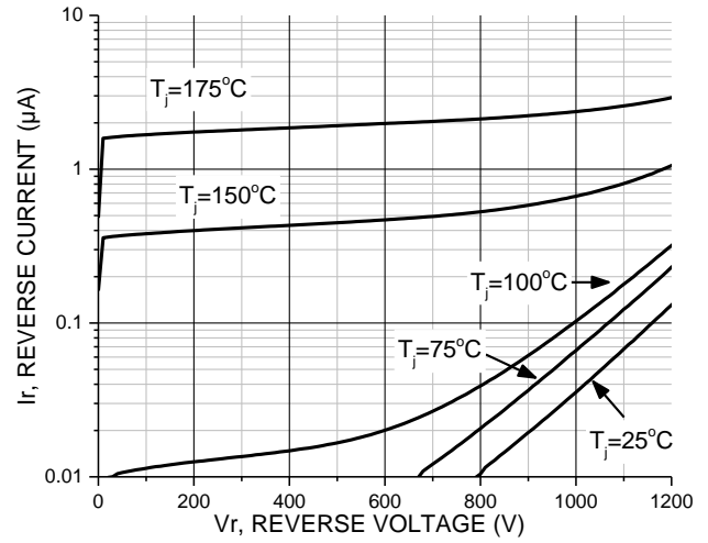
Fig. 2. Reverse Characteristics
